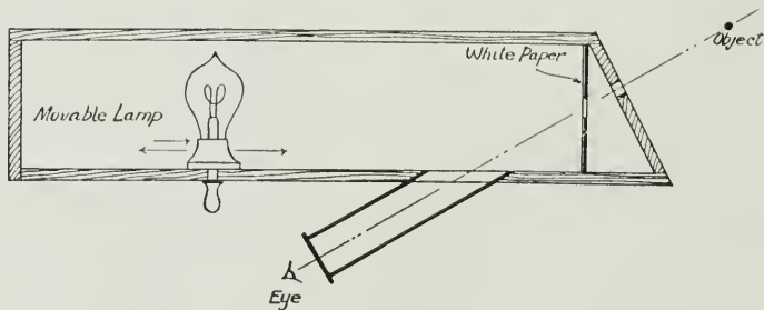
Fig. 60. Photometer to Measure Relative Brightness.
